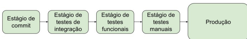
Figura 1.1: Pipeline de deployment
