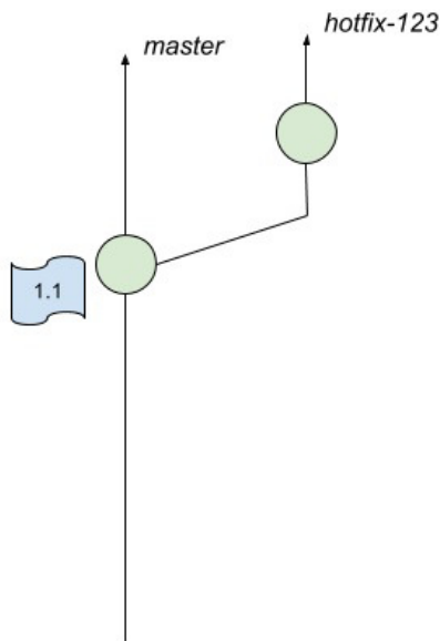
Figura 2.9: Hotfix branch
