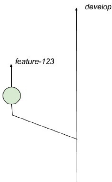
Figura 2.7: Feature branch
