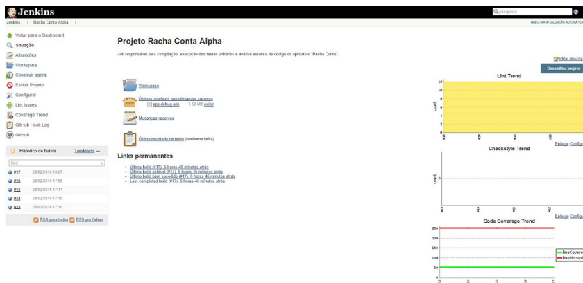
Figura 1.11: Jenkins
