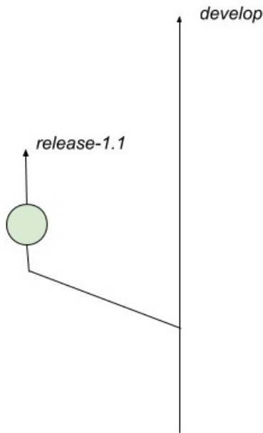
Figura 2.8: Release branch
