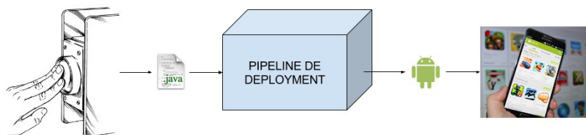
Figura 1.12: Deployment "push-button"
